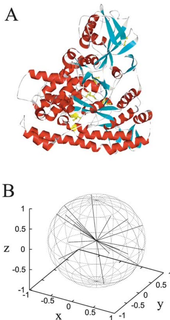
Figure 3. (A) Three-dimensional structure of the 723 residue protein malate synthase G (PDB code: 1D8C). Malate synthase G contains only six cysteines. These are highlighted in yellow including their side-chains. (B) Orientation of the 18 internuclear vectors in malate synthase G that correspond to the 18 ^1D_{NH} , ^1D_{NC'} , ^1D_{C'CA} couplings of the six cysteines. Orientations are shown in the coordinate frame of the crystal structure (A).
