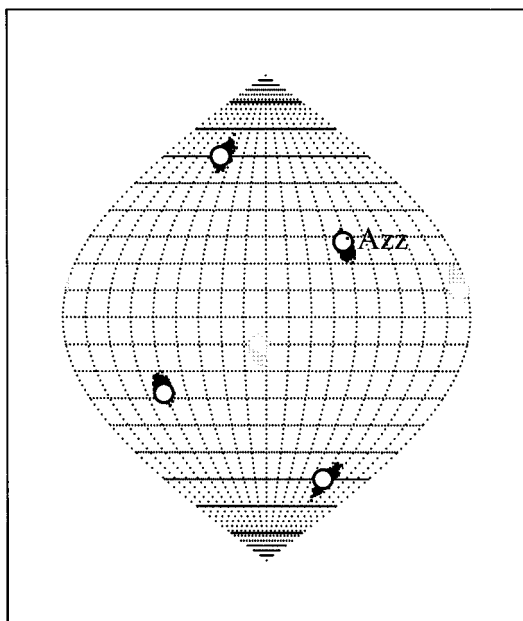
Figure 4. Orientation of the molecular alignment tensor of the 723 residue protein malate synthase G determined by exhaustive back-calculation on 18 ^1D_{NH} , ^1D_{NC'} , ^1D_{C'CA} couplings of six cysteines in MSG. The alignment tensor was determined without backbone resonance assignment. Orientations are visualized using Sauson-Flaumsteed projections (z-axis/black with label Azz; y-axis/black; x-axis/gray). Uncertainty estimates are obtained from 'structural noise Monte-Carlo simulations'. \circ Indicate the true orientation of the alignment tensor axes.
