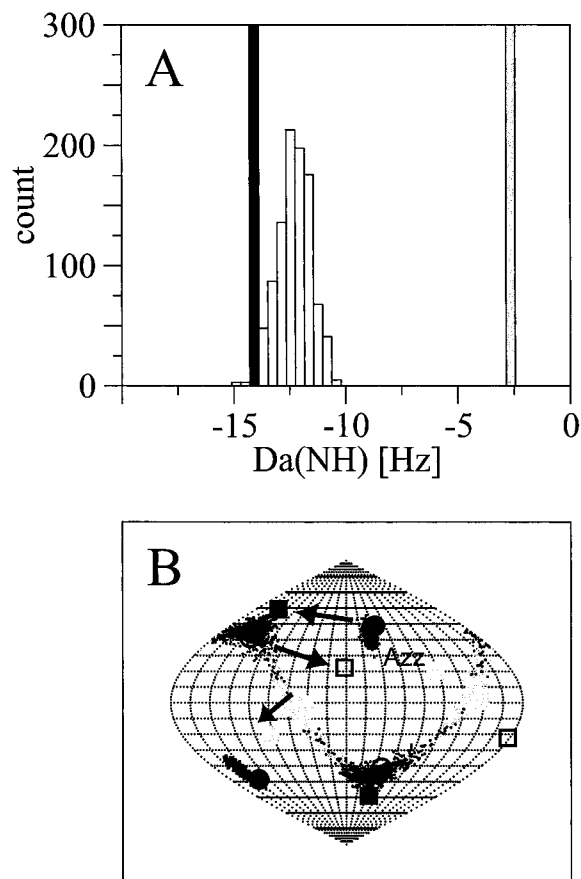
Figure 6. Comparison of the experimental alignment tensor of BAF determined by exhaustive back-calculation and alignment tensors predicted from the three-dimensional shape of homodimeric and monomeric BAF. Experimental ^1D_{NH} , ^1D_{NC'} , ^1D_{C'CA} couplings and a 1.9 Å crystal structure (PDB code: 1CI4) were used. (A) Alignment magnitude: exhaustive back-calculation (white); homodimeric shape-prediction (black); monomeric shape-prediction (gray). (B) Alignment tensor orientation (z-axis/black with label Azz; y-axis/gray; x-axis/black): Dots (exhaustive back-calculation), ● (homodimeric shape-prediction), ■ (monomeric shape-prediction). The change in orientation when going from the homodimeric to the monomeric structure is indicated by arrows.
