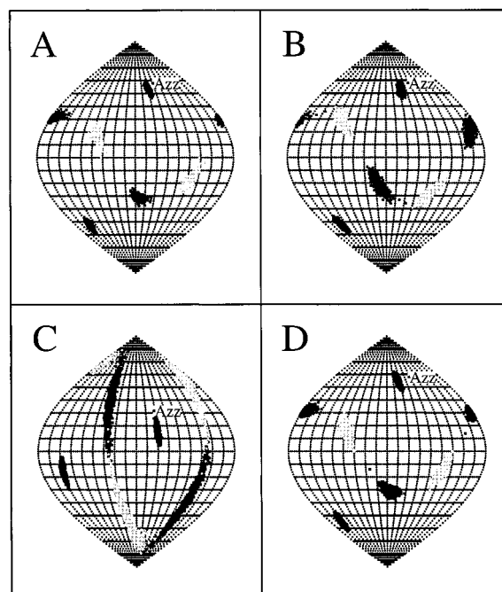
Figure 1. Orientation of the molecular alignment tensor of ubiquitin determined without knowledge of its backbone assignment using exhaustive back-calculation on ILE (A), LEU (B), ARG (C) and ILE-ARG (D). Experimental ^1D_{NH} , ^1D_{NC'} , ^2D_{HNC'} couplings observed in 30:10 DMPC:DHPC bicelles and a 1.8 Å crystal structure (PDB code: 1UBQ) are used (Table 2). Orientations are visualized using Sauson-Flaumsteed projections (z-axis/black with label Azz; y-axis/black; x-axis/gray). Uncertainty estimates are obtained from 'structural noise Monte-Carlo simulations'.
