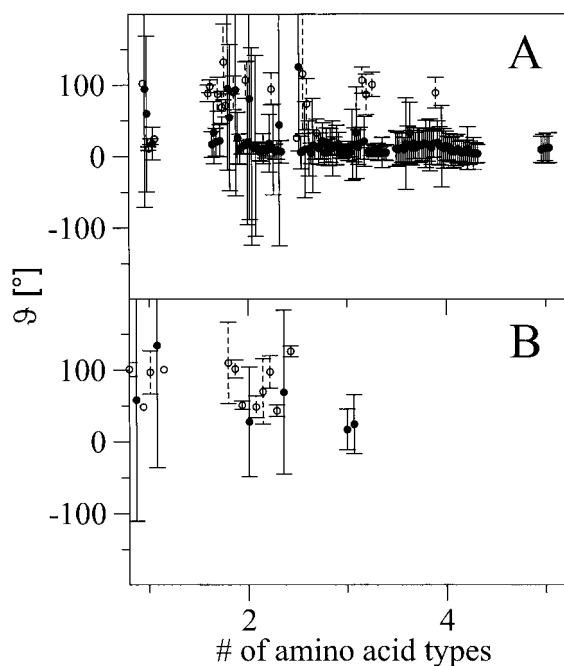
Figure 5. Deviation of alignment tensors determined by exhSVD from the correct orientation for an increasing number of selected amino acid types. Only ^1D_{NH} couplings from a single alignment medium are used. (A) exhSVD results on ubiquitin. (B) exhSVD results on maltodextrin-binding protein. Differences in tensor orientations are expressed by the generalized angle \vartheta (Sass et al., 2001). Uncertainty estimates are obtained from 'structural noise Monte-Carlo simulations'. \bullet and \circ indicate exhSVD results where the error in the tensor orientation is smaller or larger than the estimated uncertainty, respectively. Note that in (A) (ubiquitin) only the worst case data are shown, i.e. where at least one amino acid type is strongly influenced by errors in the crystal structure.
