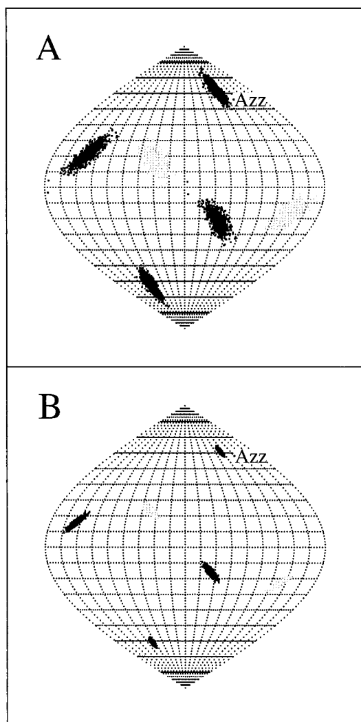
Figure 2. Orientation of the molecular alignment tensor of the 370 residue maltodextrin-binding protein (MBP) determined without (A) and with (B) knowledge of its backbone assignment. (A) Exhaustive back-calculation using 17 experimental ^1D_{NH} , ^1D_{NC'} , ^1D_{C'CA} couplings of six observable tryptophans in MBP (Table 4); (B) regular SVD with 279 ^1D_{NH} couplings. Orientations are visualized using Sauson-Flaumsteed projections (z-axis/black with label Azz; y-axis/black; x-axis/gray). Uncertainty estimates are obtained from 'structural noise Monte-Carlo simulations'.
